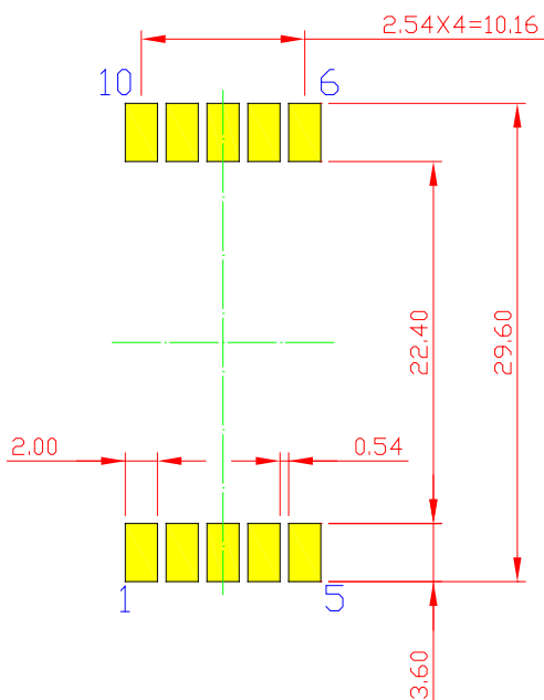
Recommended Soldering Pattern
