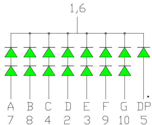
OPS-S8011PG-GW (Common Cathode)
