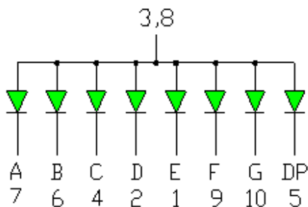
OPS-S5620SPG-GW ( Common Anode )
