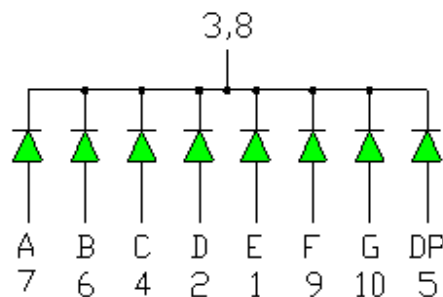
OPS-S5621SPG-GW ( Common Cathode )
