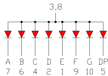
OPS-S5110LE-GW (Common Anode)
