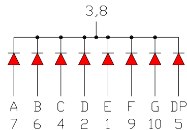
OPS-S5111LE-GW (Common Cathode)
