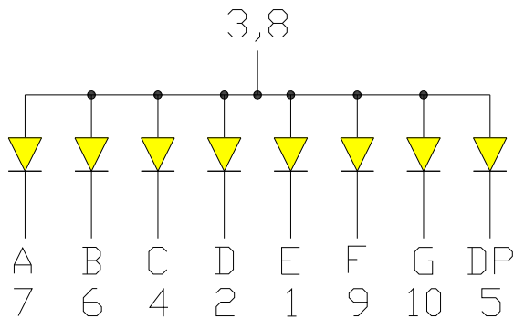
OPS-S4010LY-GW ( Common Anode )
