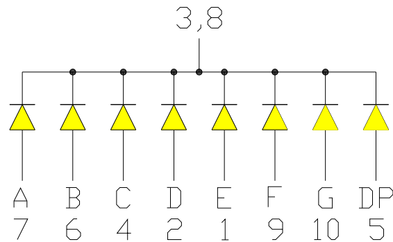
OPS-S4011LY-GW ( Common Cathode )
