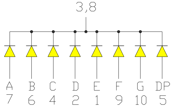
OPS-S3911LY-GW (Common Cathode)
