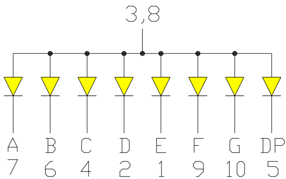
OPS-S3910LY-GW (Common Anode)
