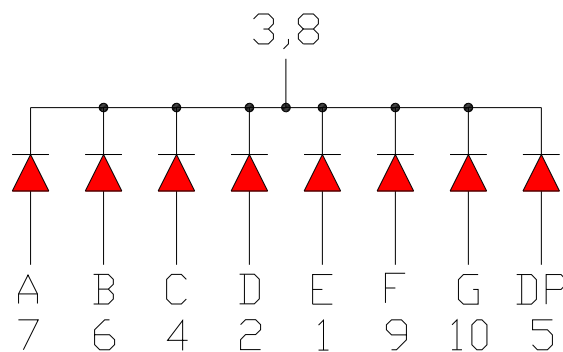
Common Cathode (OPS-S3011LR-GW)
