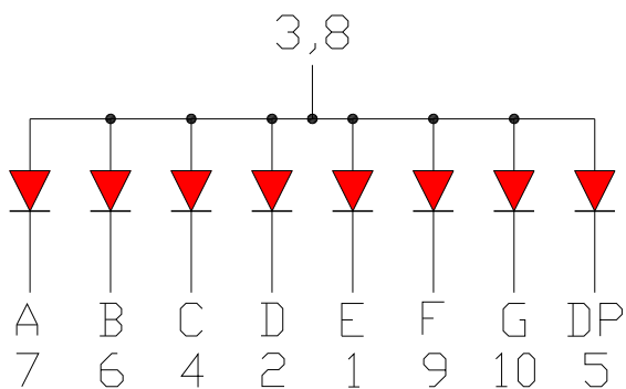
Common Anode (OPS-S3010LR-GW)
