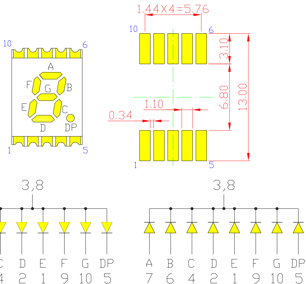
OPS-S2010LY-GW ( Common Anode )
