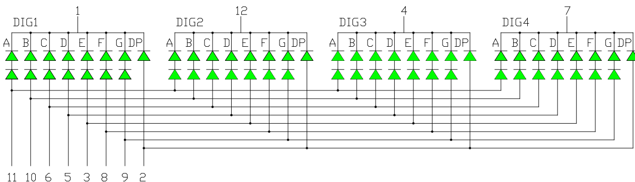
OPS-Q8011PG-GW (Common Cathode)
