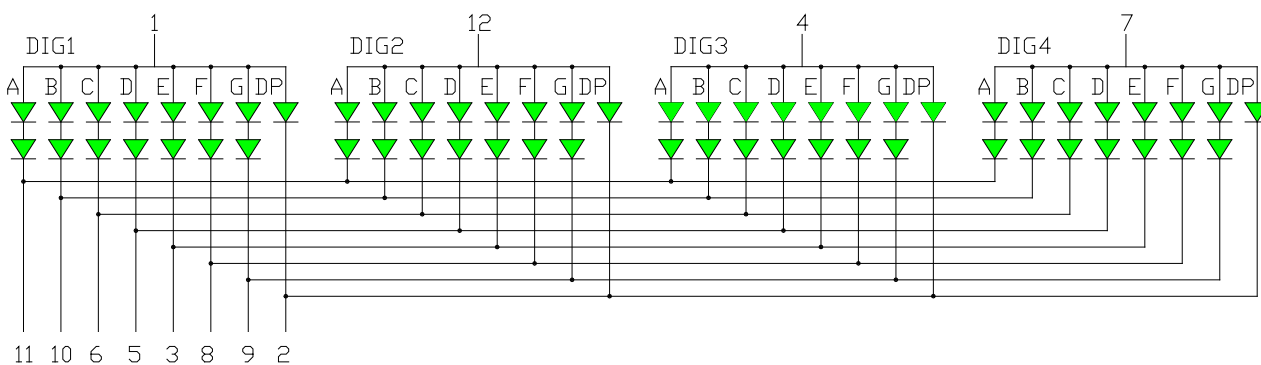
OPS-Q8010PG-GW (Common Anode)
