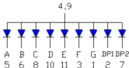
12 PIN No Connect OPS-S2812SB-GW (Common Anode)
