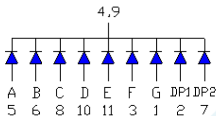
12 PIN No Connect OPS-S2811SB-GW (Common Cathode)
