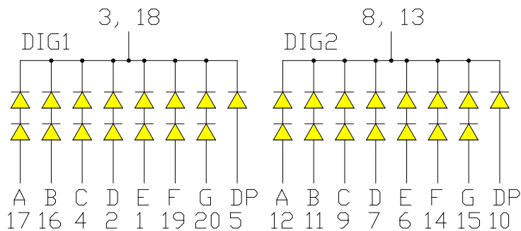
OPS-D8011LY-GW (Common Cathode)
