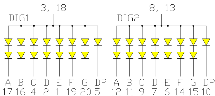
OPS-D8010LY-GW (Common Anode)
