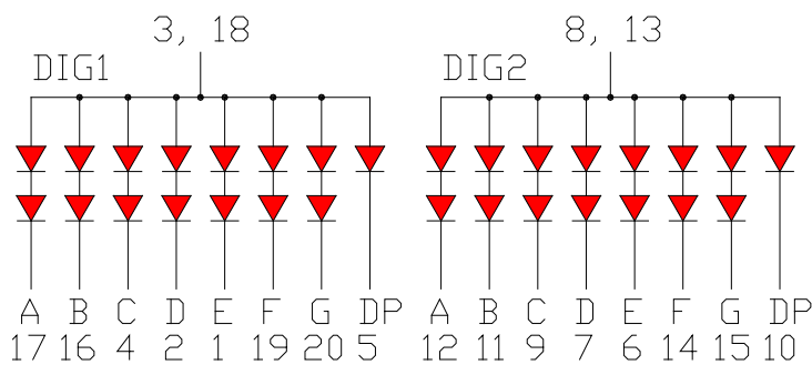
OPS-D8010LE-GW (Common Anode)
