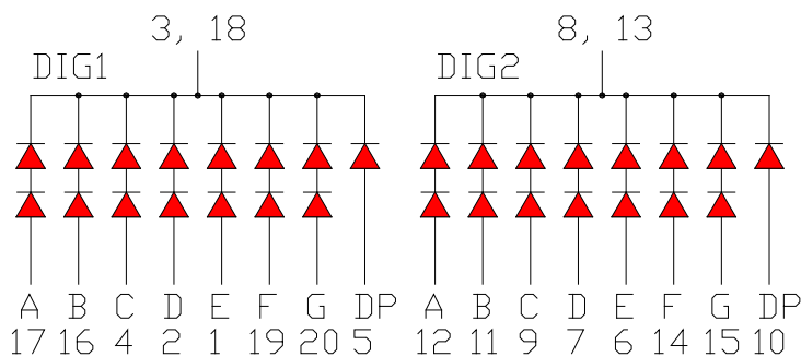
OPS-D8011LE-GW (Common Cathode)
