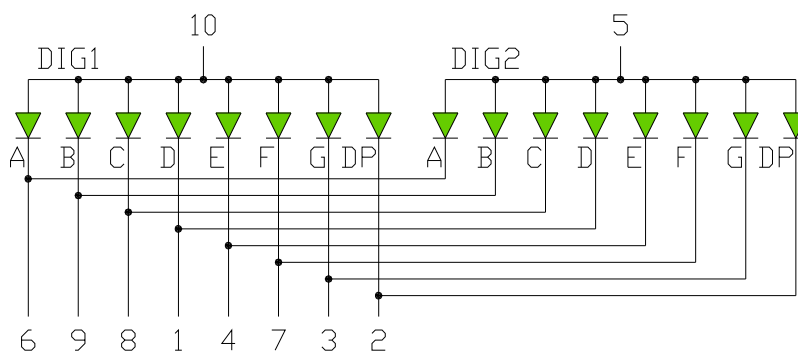
OPS-D5110YG-GW (Common Anode)
