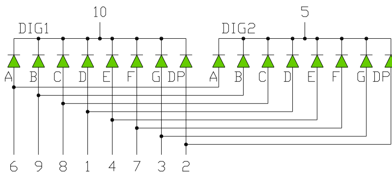
OPS-D5111YG-GW (Common Cathode)
