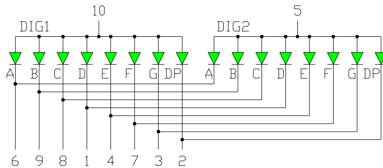
OPS-D5110PG-GW (Common Anode)
