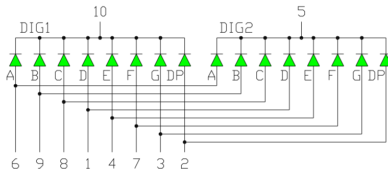
OPS-D5111PG-GW (Common Cathode)
