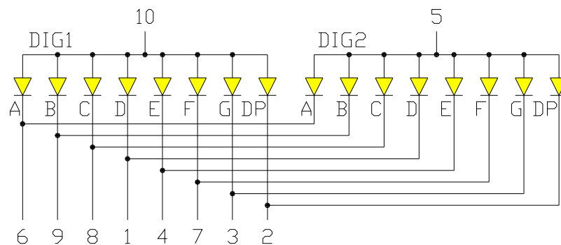
OPS-D5110LY-GW (Common Anode)
