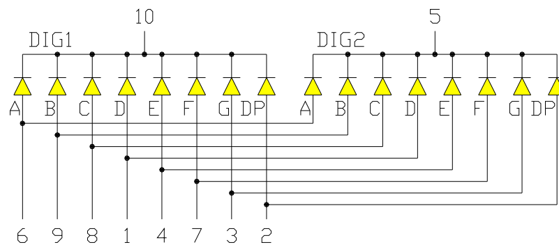
OPS-D5111LY-GW (Common Cathode)
