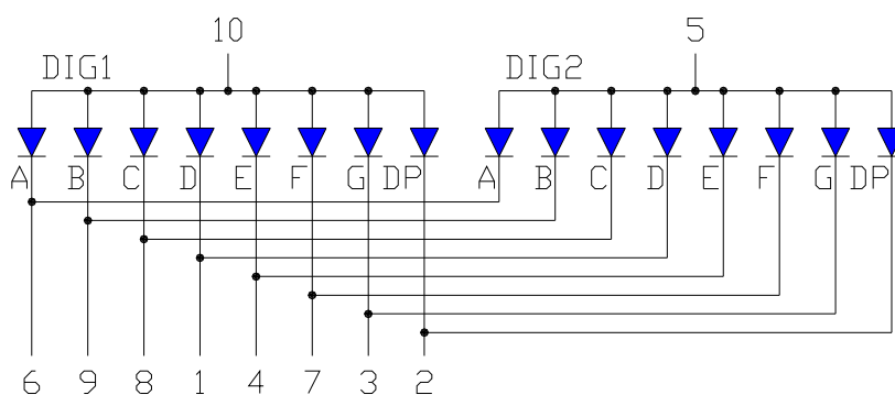
OPS-D5110LB-GW (Common Anode)
