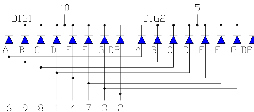
OPS-D5111LB-GW (Common Cathode)
