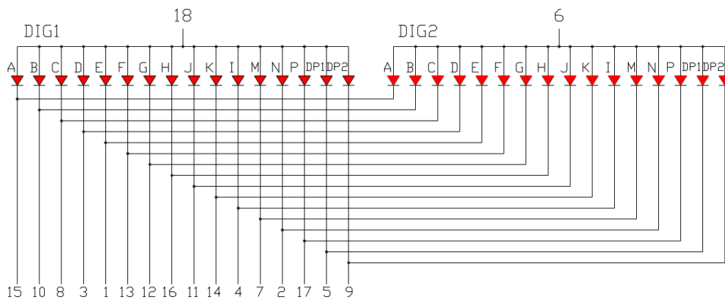
OPS-AD5640LR-GW (Common Anode)
