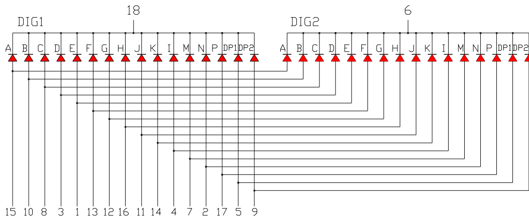
OPS-AD5641LR-GW (Common Cathode)
