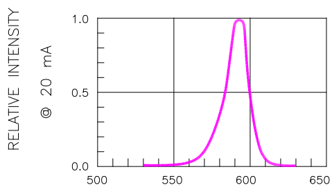
Fig.5 RELATIVE INTENSITY VS. WAVELENGTH
